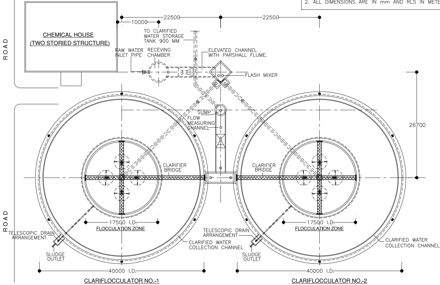
LAYOUT OF EXISTING PLANT.
