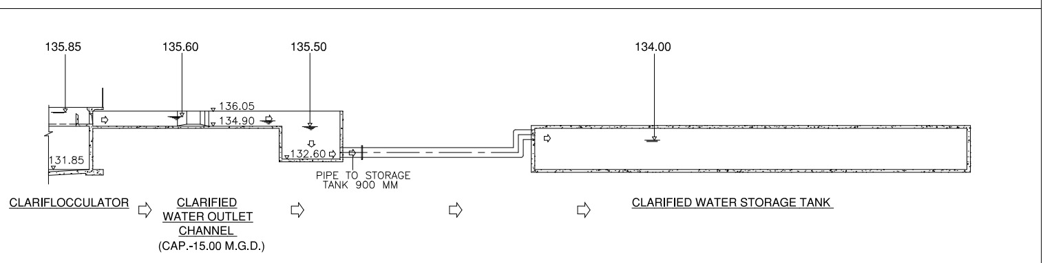
HYDRAULIC FLOW DIAGRAM OF THE EXISTING PLANT.
