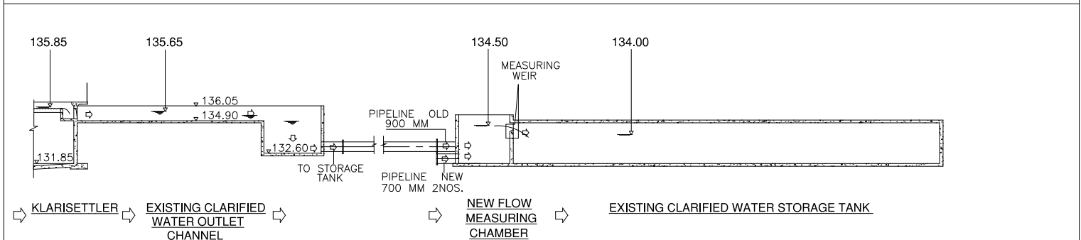
HYDRAULIC FLOW DIAGRAM OF THE AUGMENTED PLANT.
