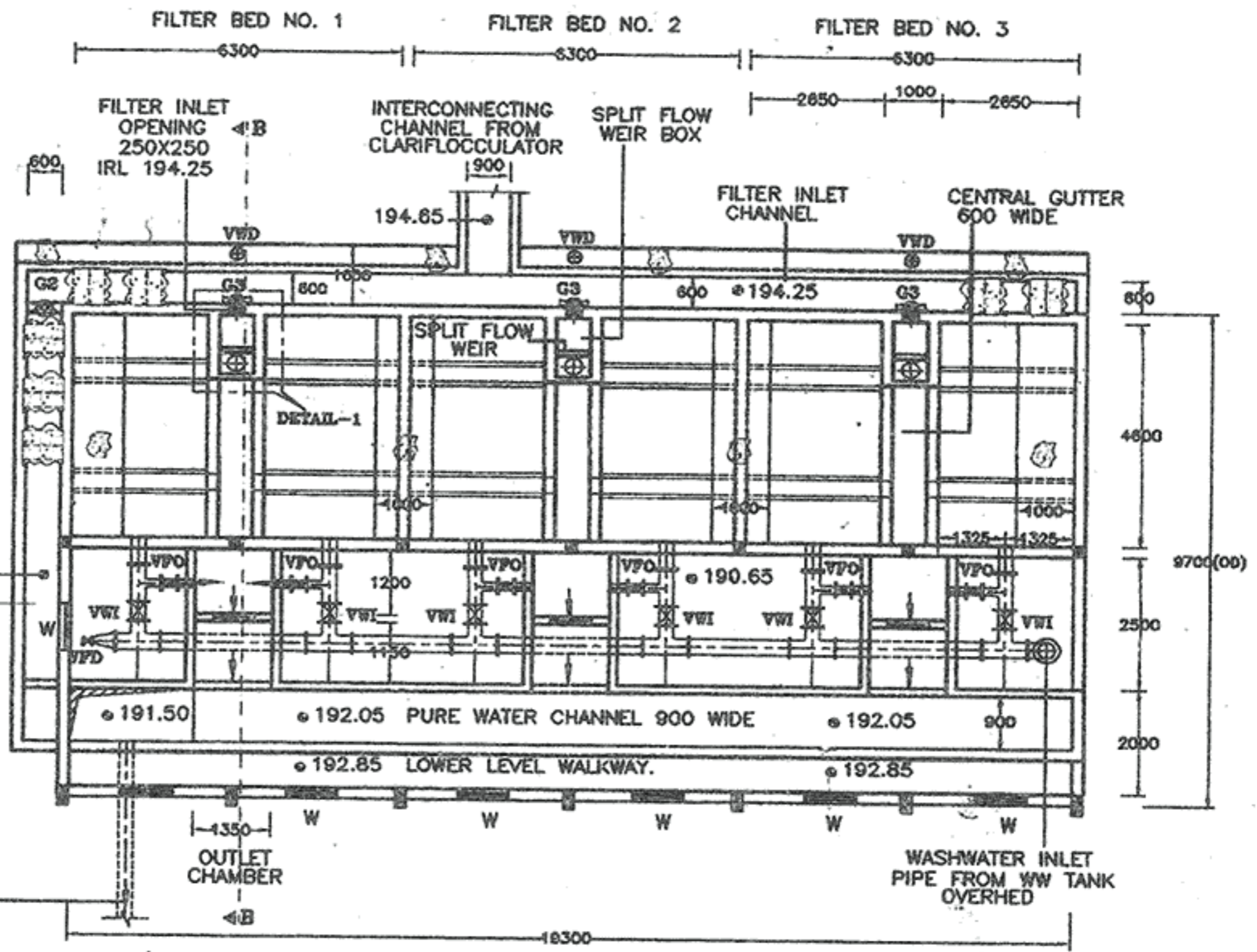
PLAN OF FILTER BEDS
