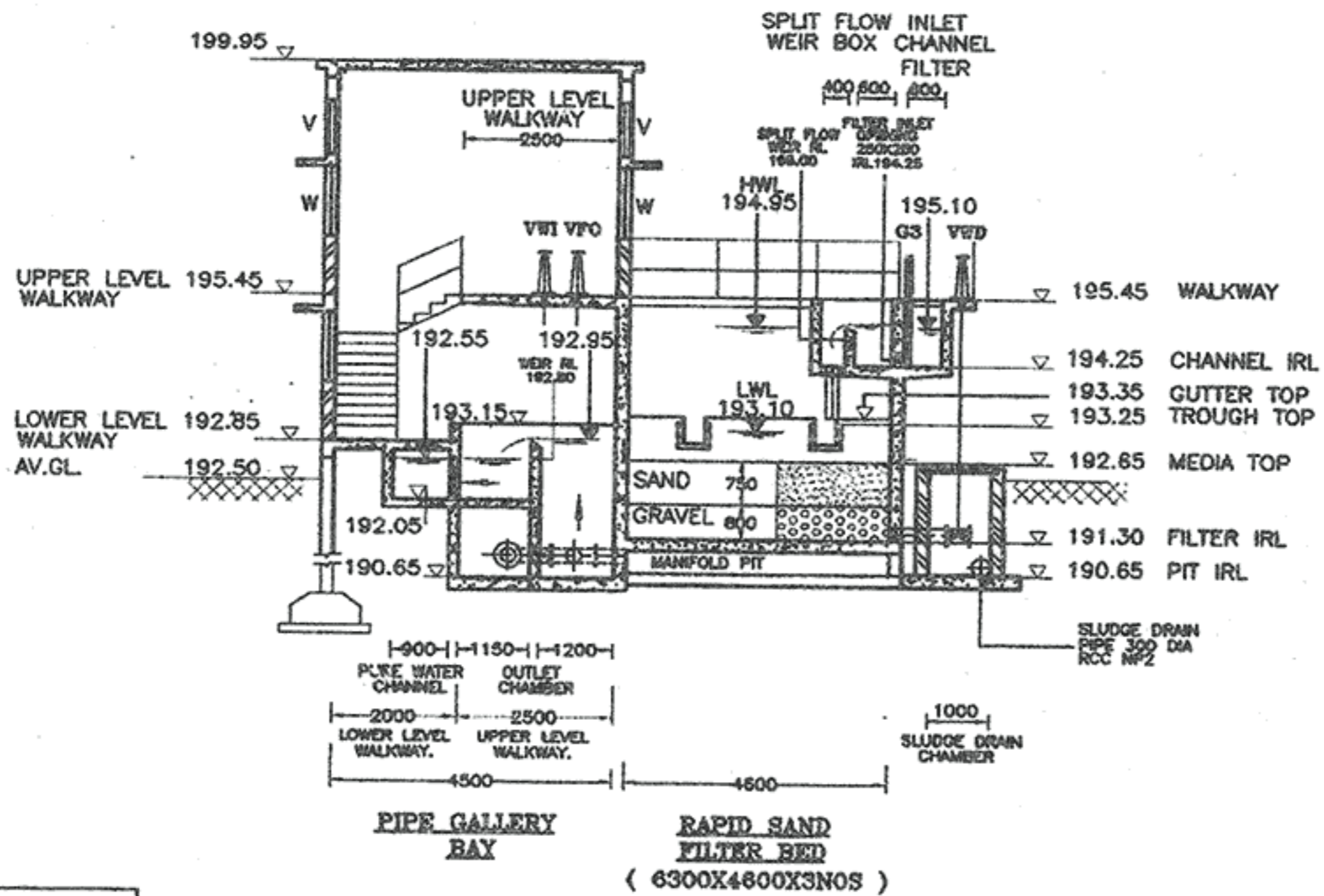
SECTION B-B
