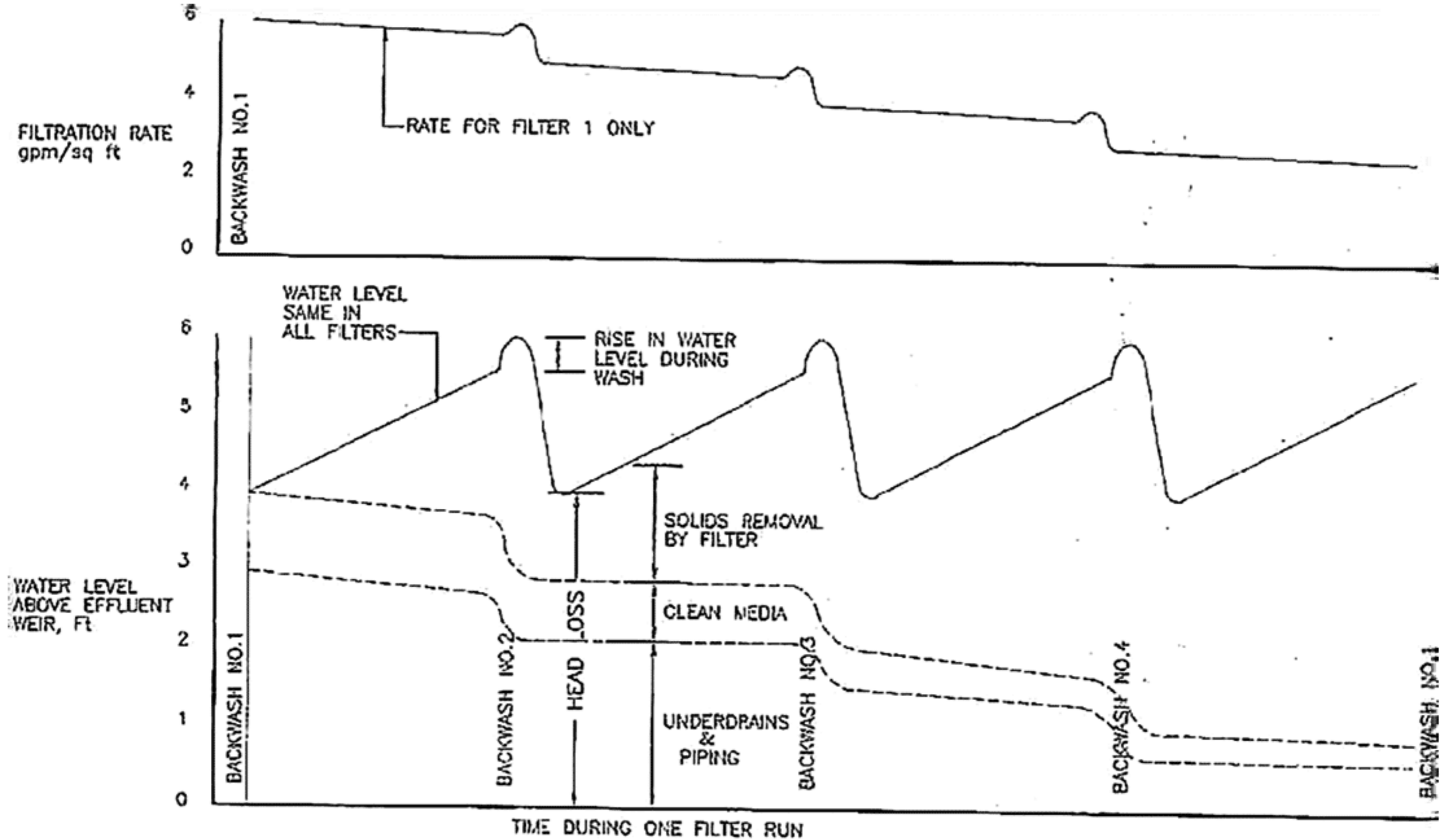
VARIABLE DECLINING RATE FILTRATION—FILTRATION RATE, HEAD LOSS, AND WATER LEVEL DURING ONE FILTER RUN IN A PLANT HAVING FOUR FILTERS
